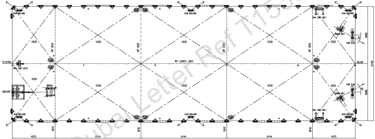
MAIN DECK ARRANGEMENT PLAN
