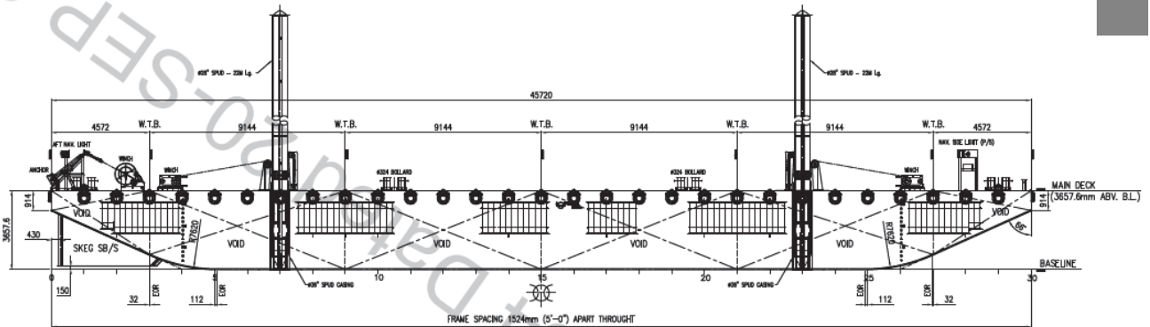
OUTBOARD PROFILE
