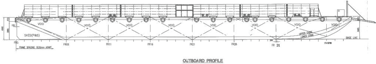
OUTBOARD PROFILE
