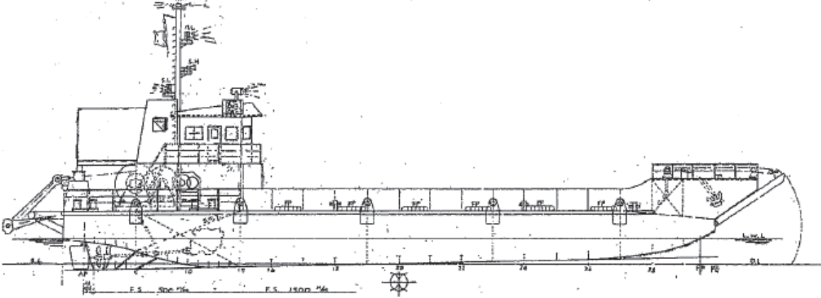
SIDE VIEW
