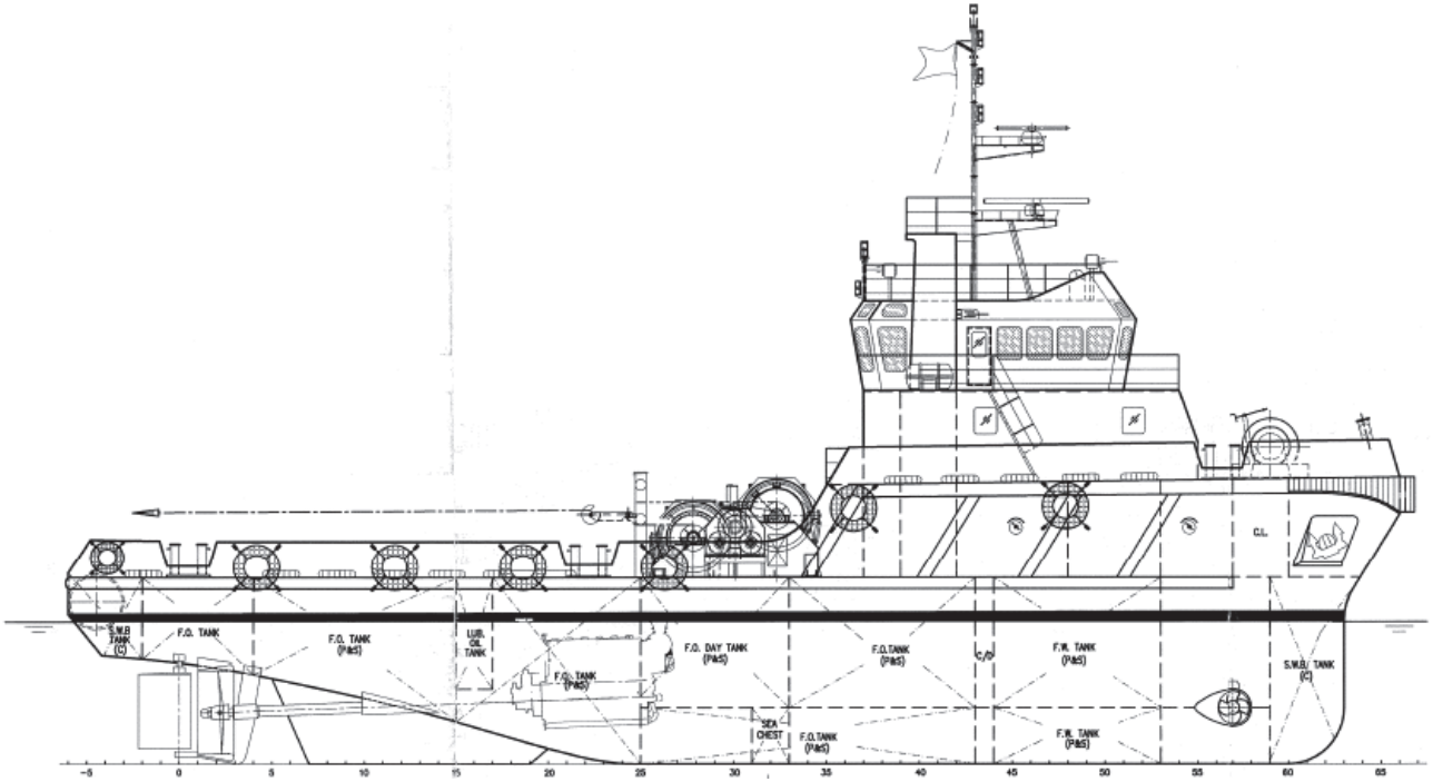
SIDE VIEW
