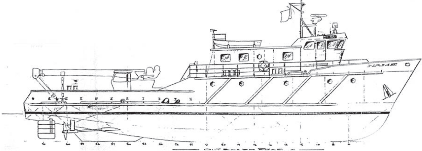
SIDE VIEW DECK LEVEL
