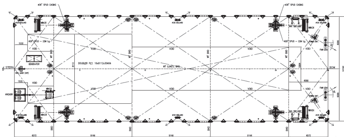
MAIN DECK ARRANGEMENT PLAN
