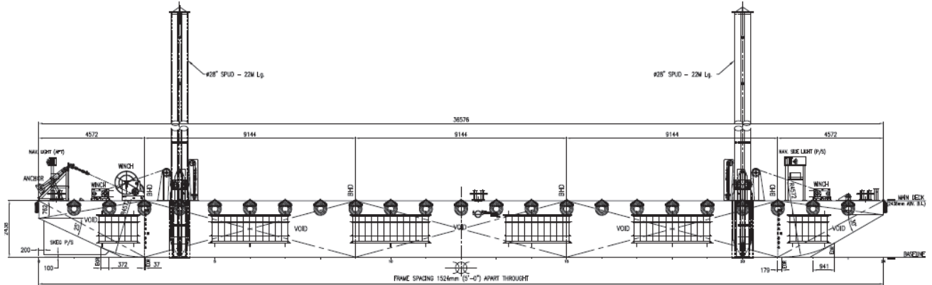
OUTBOARD PROFILE
