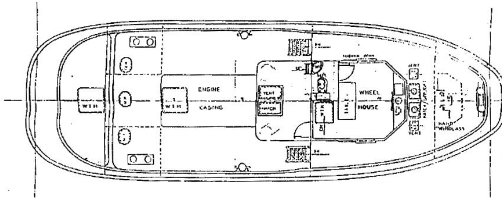
MAIN DECK VIEW
