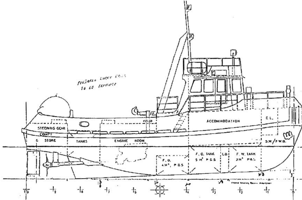
SIDE VIEW
