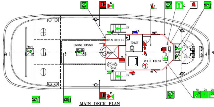
MAIN DECK VIEW
