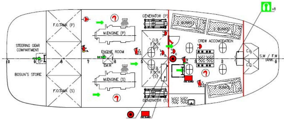
BELOW MAIN DECK VIEW
