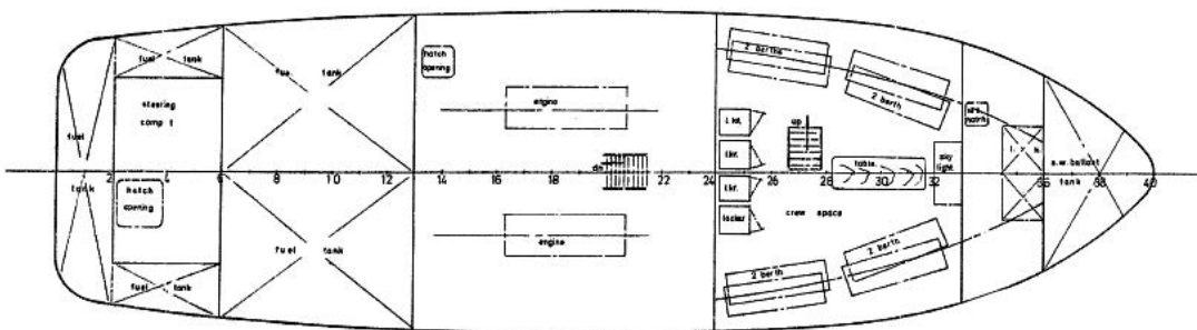
BELOW MAIN DECK VIEW
