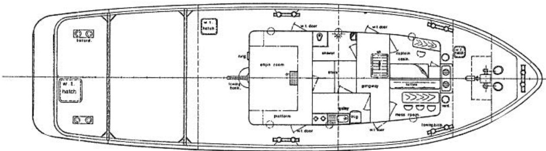
MAIN DECK VIEW
