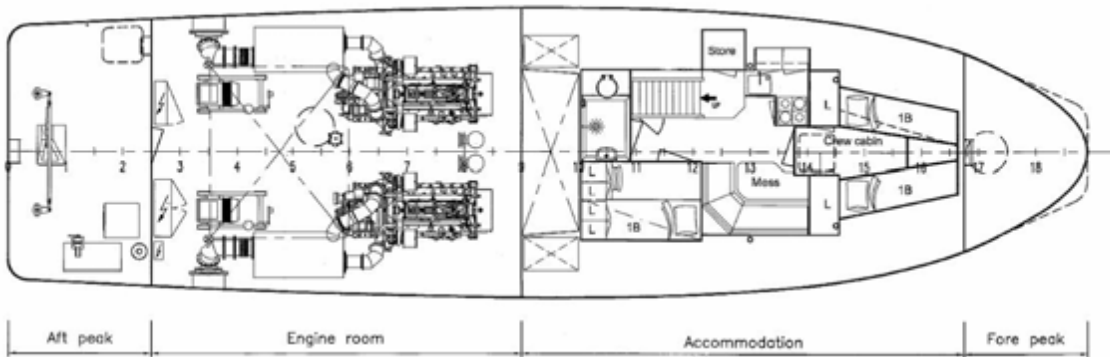
BELOW MAIN DECK VIEW
