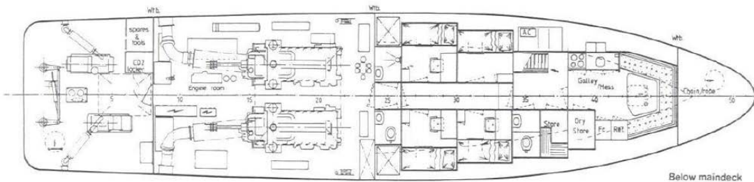
BELOW MAIN DECK VIEW
