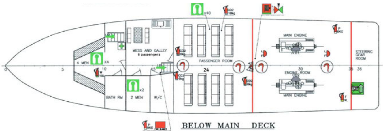
BELOW MAIN DECK VIEW
