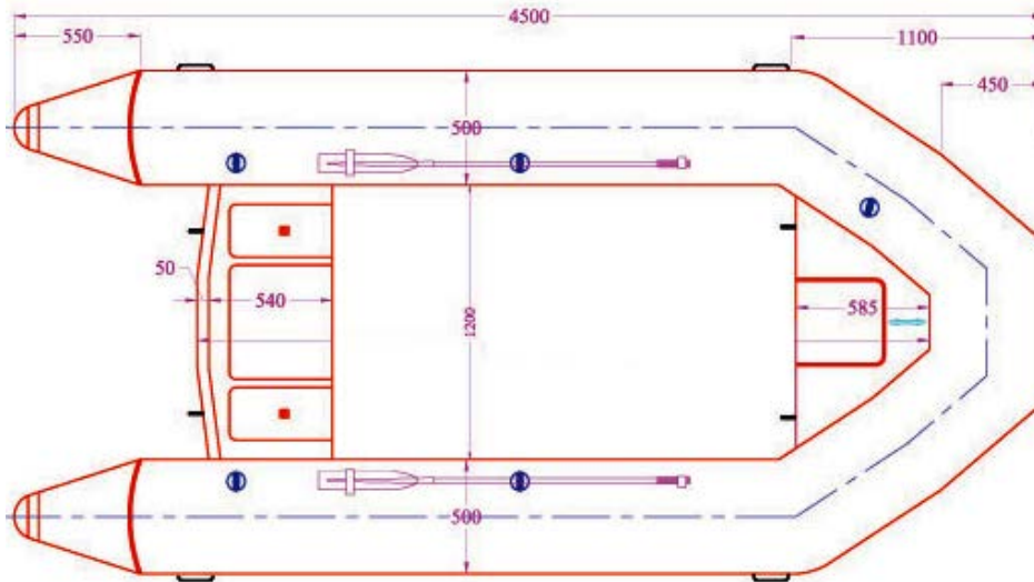
TOP VIEW DECK LEVEL
